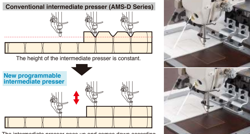
The intermediate presser goes up and comes down according to the material thickness.
